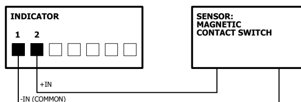
CONNECTION DETAIL
